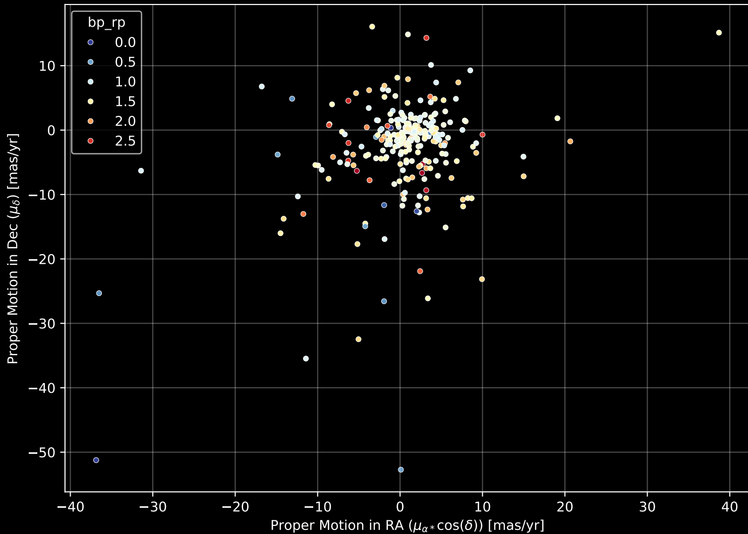
APOGEE DR17 Field: [139+27_btx] Proper Motion Diagram (n= 259)
