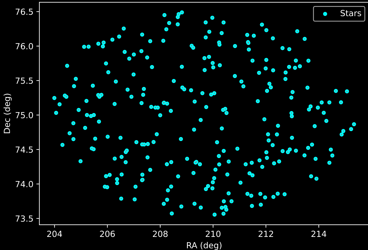
APOGEE DR17 Field: [139+27_btx] Proper Motion Vectors for Gaia Star Field (n= 259)
