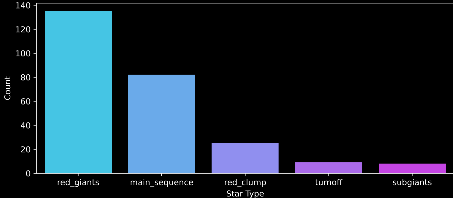
APOGEE DR17 Field: [139+27_btx] Count plot of Star Type
