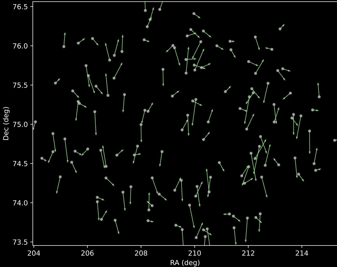
APOGEE DR17 Cluster 5 Proper Motion Vectors (n=133)
