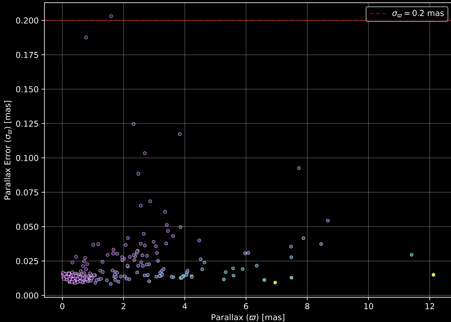
APOGEE DR17 Field: [139+27_btx] Parallax Quality (n= 259)
