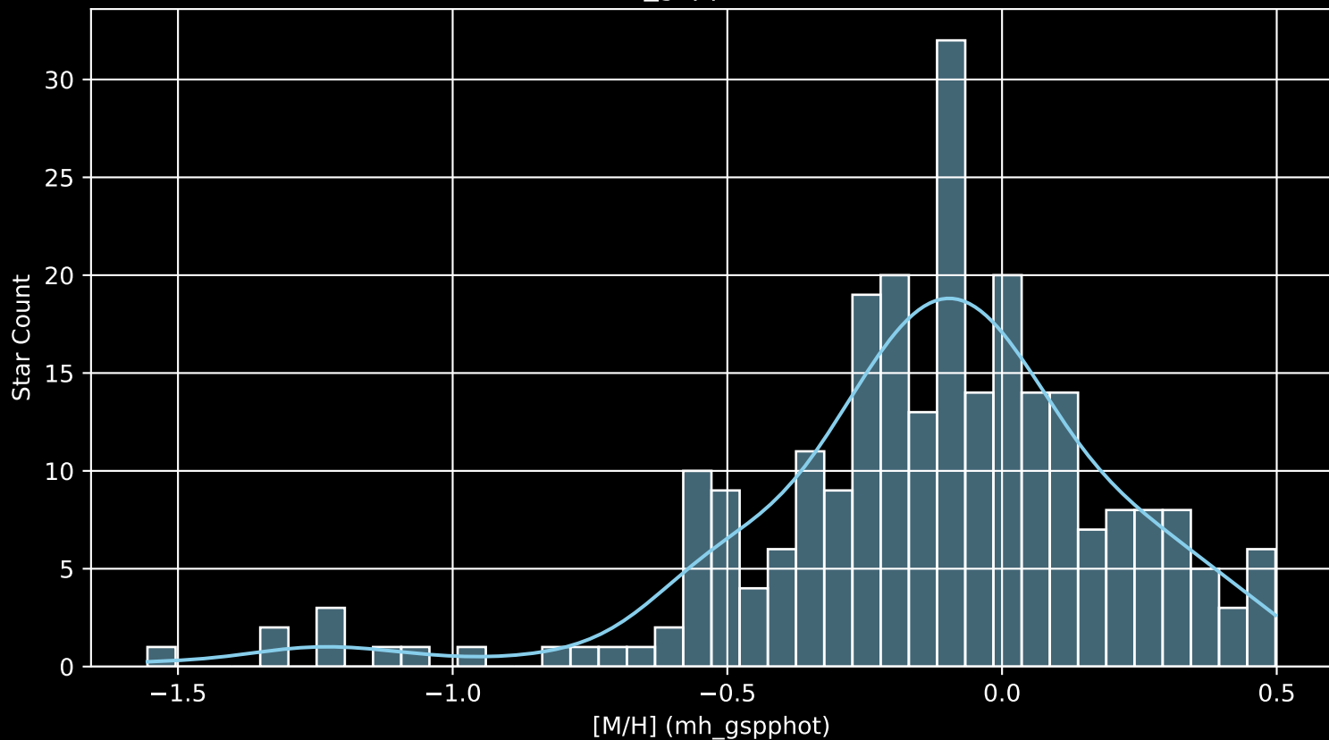
APOGEE DR17 Field: [139+27_btx [M/H] (mh_gspphot) (n= 255)
