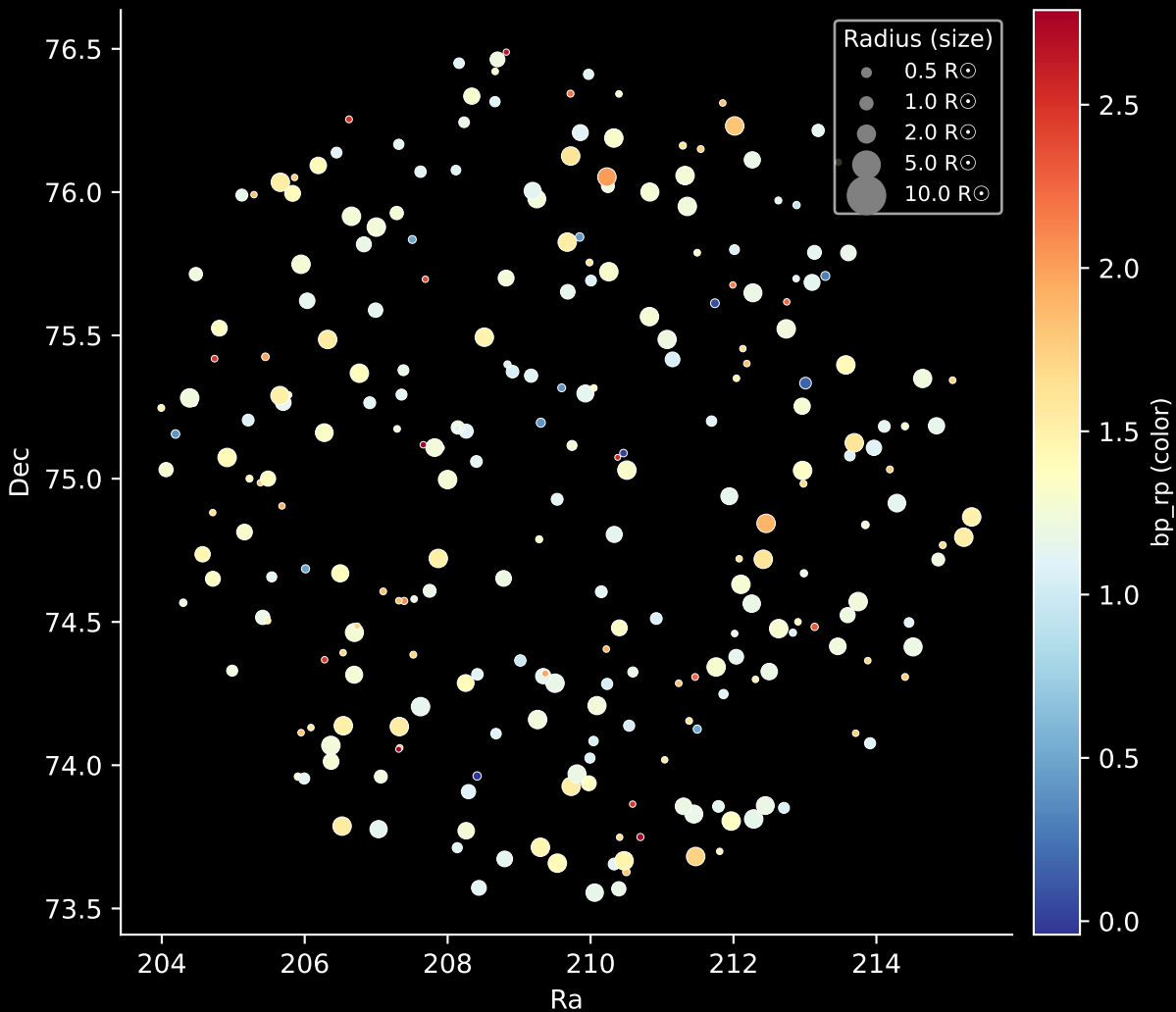
APOGEE DR17 Field: [139+27_btx] Stars: 259
