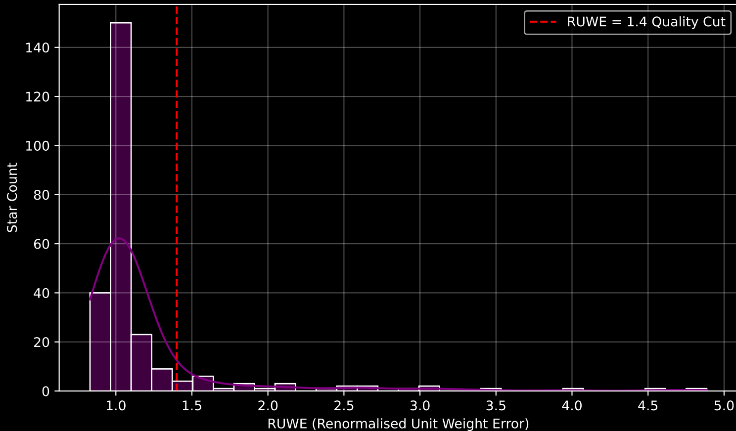
GAPOGEE DR17 Field [139+27_btx] RUWE Distribution (n= 252)
